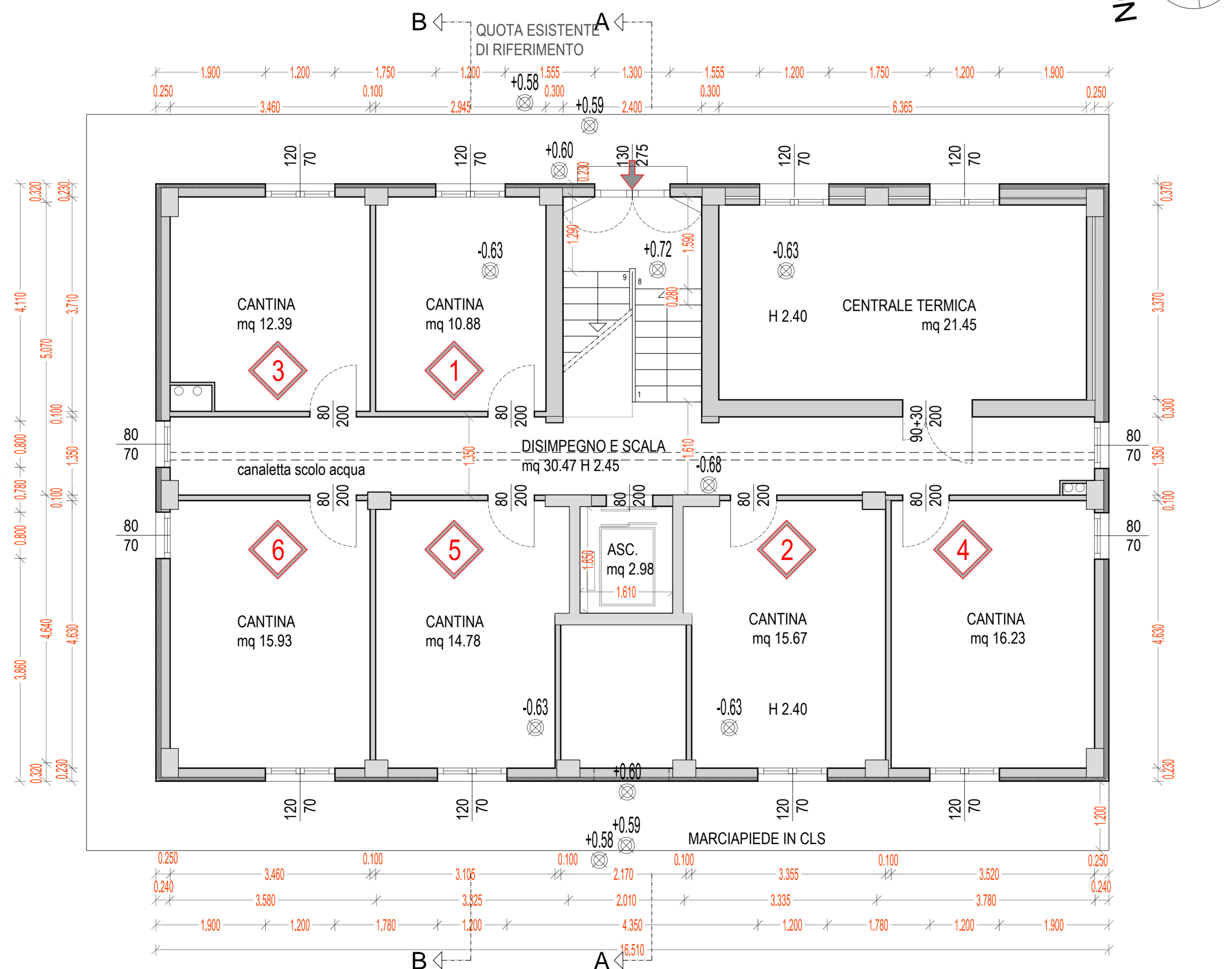
PIANO SEMIINTERRATO
